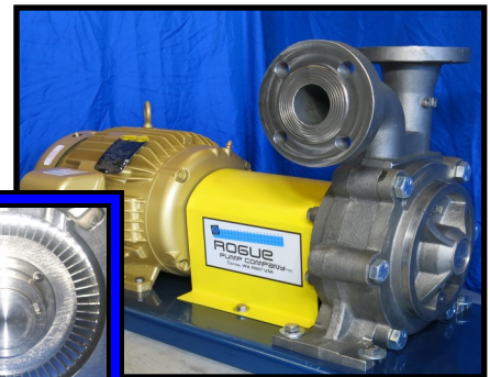
PEWE uses Rogue MAX RGT ® regenerative turbine pumps.
